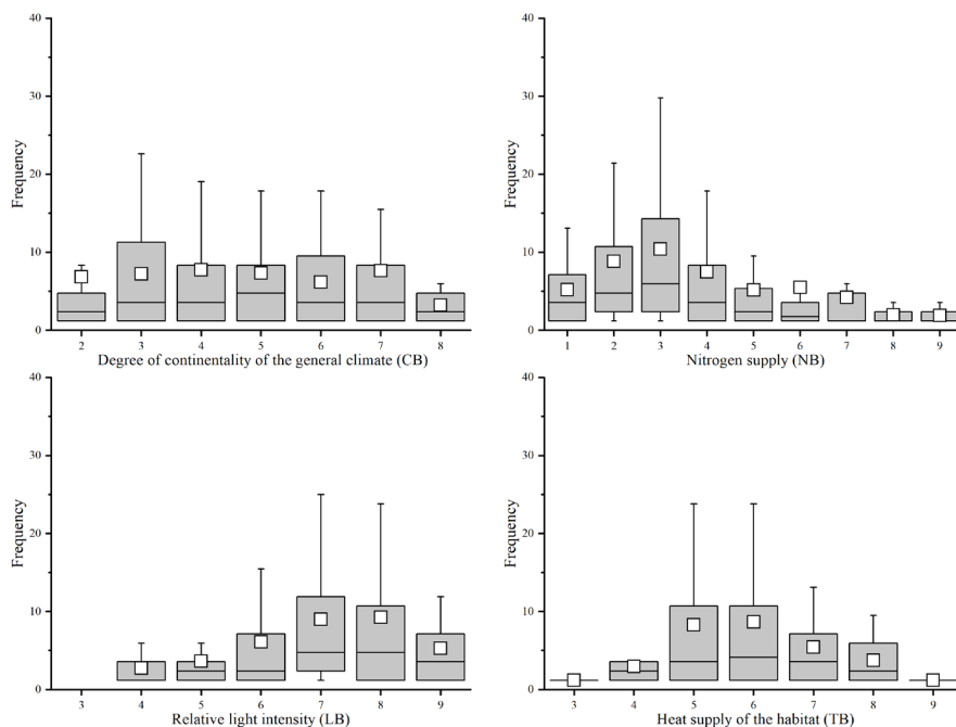
Fig. 3. Distribution of species frequency (mean cover \pm S.E.) between the indicator values of continentality (CB), nitrogen supply (NB), light intensity (LB) and heat supply of the habitat (TB). Boxes are 25% – 75% percentiles, whiskers are outliers, horizontal lines are median values, open squares are mean values.
