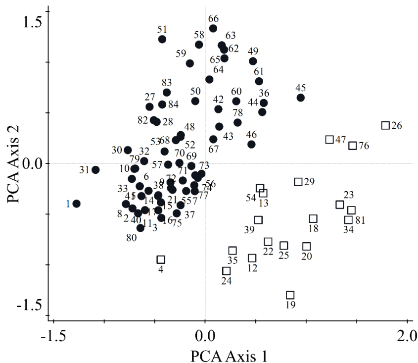
Fig. 4. Ordination of plots containing Himatoglossum adriaticum . Ordination plot was based on percentage cover of species in the sampled plots using principal component rotation of NMDS axes. Notations: open square = plots with high cover of trees and shrubs; filled circle = plots with low cover of trees and shrubs.
