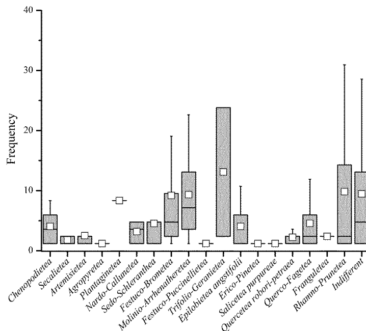
Fig. 2. Distribution of species frequency between plant phytosociological units (BORHIDI 1995). Boxes are 25% – 75% percentiles, whiskers are outliers, horizontal lines are median values, open squares are mean values.
